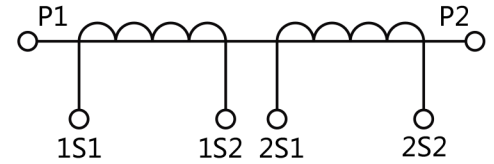
Double winding
